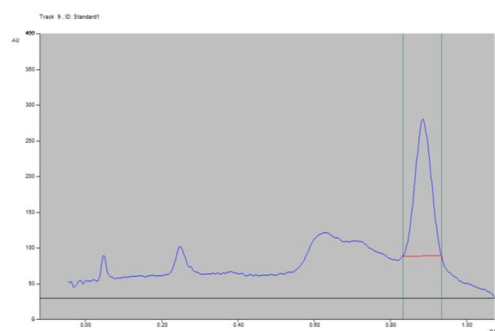
Fig.52: HPTLC Chromatograph of Tricel (Chlorpyrifos)
