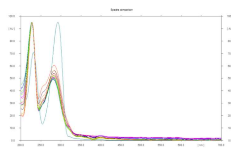
Fig.53: HPTLC Spectra of different treatments
