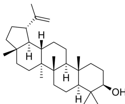
Chemical structure of Lupeol
